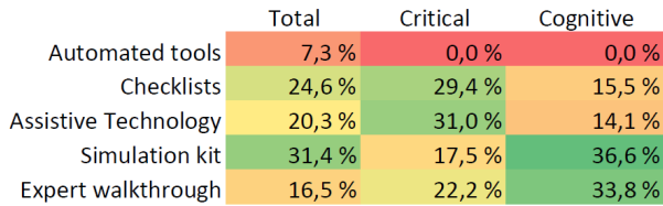
FIGURE 2. HEAT MAP OF ERRORS FOUND WITH THE VARIOUS TESTING METHOD GROUPS.
